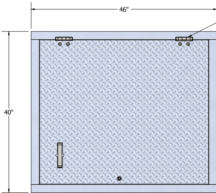
PLAN VIEW
